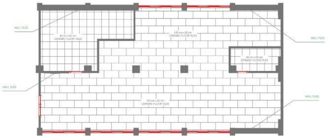
WALL & FLOOR FINISH LAYOUT
