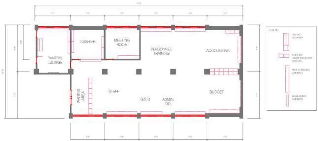
FLOOR PLAN W/ BUILT-IN FURNITURE LAYOUT
