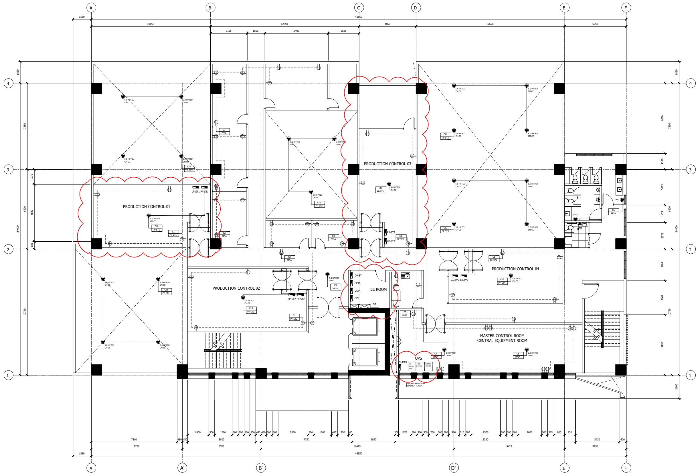
THIRD FLOOR 01 POWER LAYOUT E-208.0 SCALE: 1:100m
